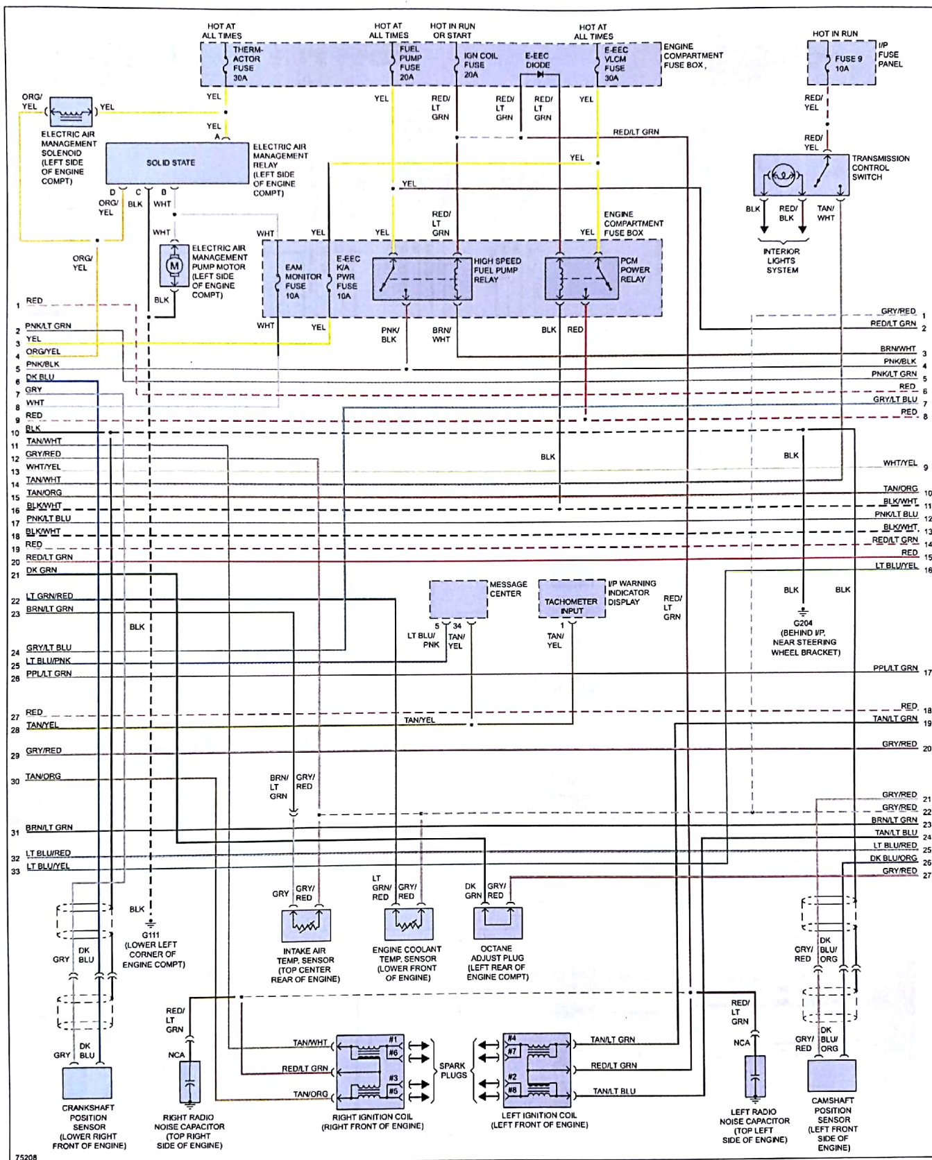
Fig 2: 4.6L, Engine Performance Circuits (2 of 3)
