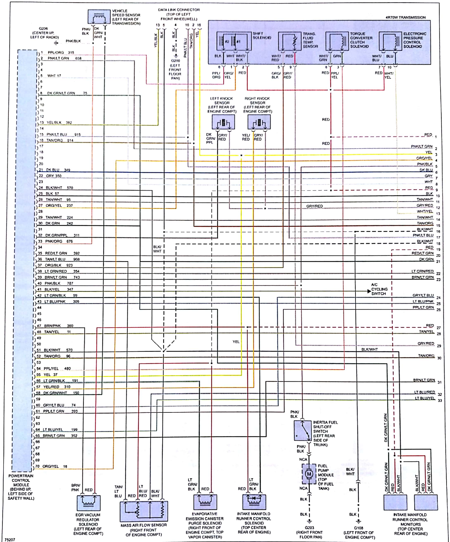
Fig 1: 4.6L, Engine Performance Circuits (1 of 3)
