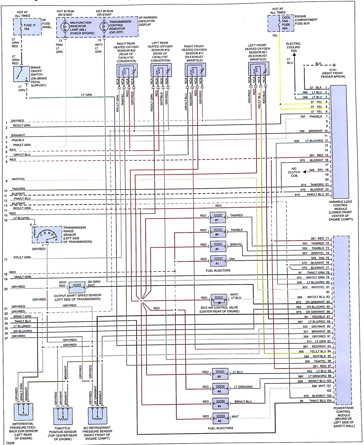
Fig 3: 4.6L, Engine Performance Circuits (3 of 3)
